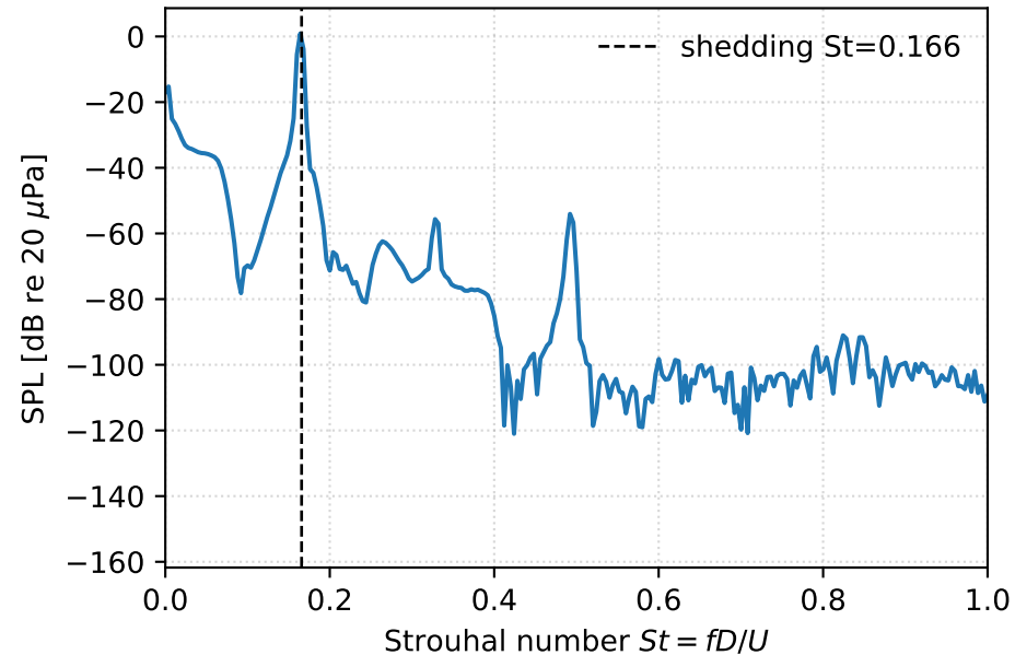
Far-field spectrum (mic_274)
