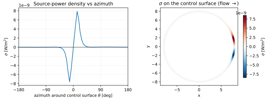
Figure 3: Source-power density \sigma on the permeable control surface ( r = 8D ) at the shedding tone: (left) azimuthal profile around the surface; (right) \sigma over the surface (mean flow left to right). The density localizes to the downstream wake-crossing sector and is signed, integrating to the far-field radiated power \oint \sigma dS = P to machine precision.
