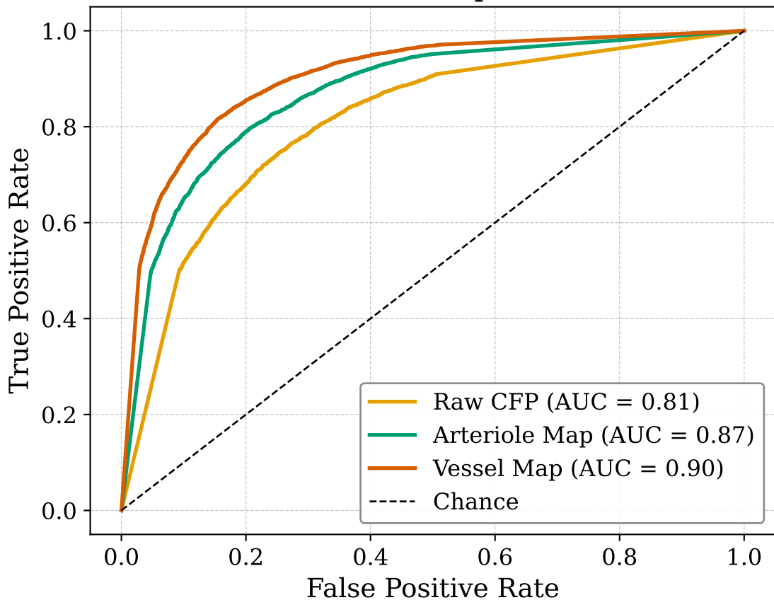
AUROC Comparison
