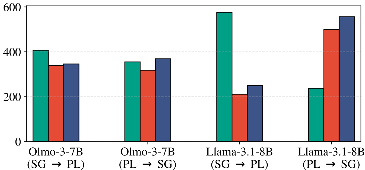
Subspace Dimension
