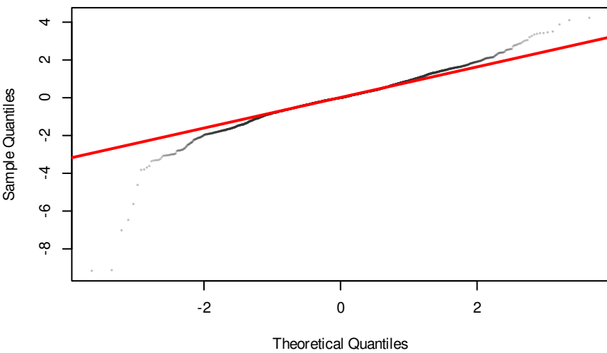
K=3 (4 random effects) — normal Q-Q
