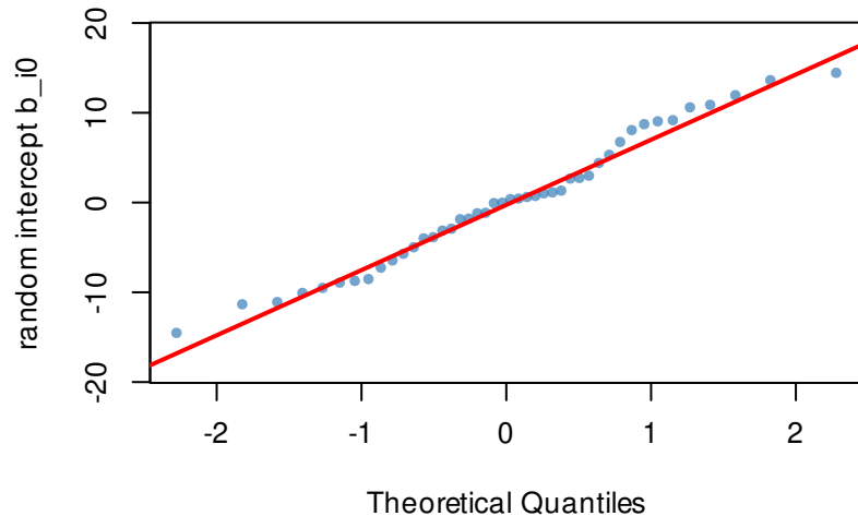
K=5: sd(b_i0) 6.48 | 6 rand.eff
