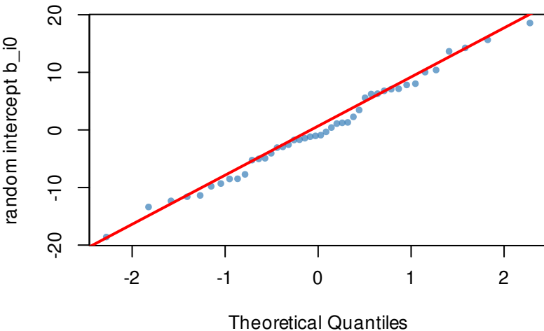
K=4: sd(b_i0) 7.53 | 5 rand.eff
