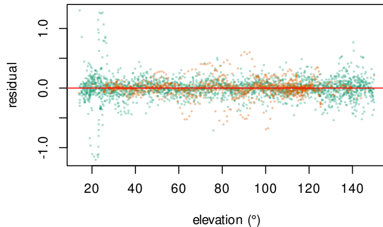
Residuals vs x
