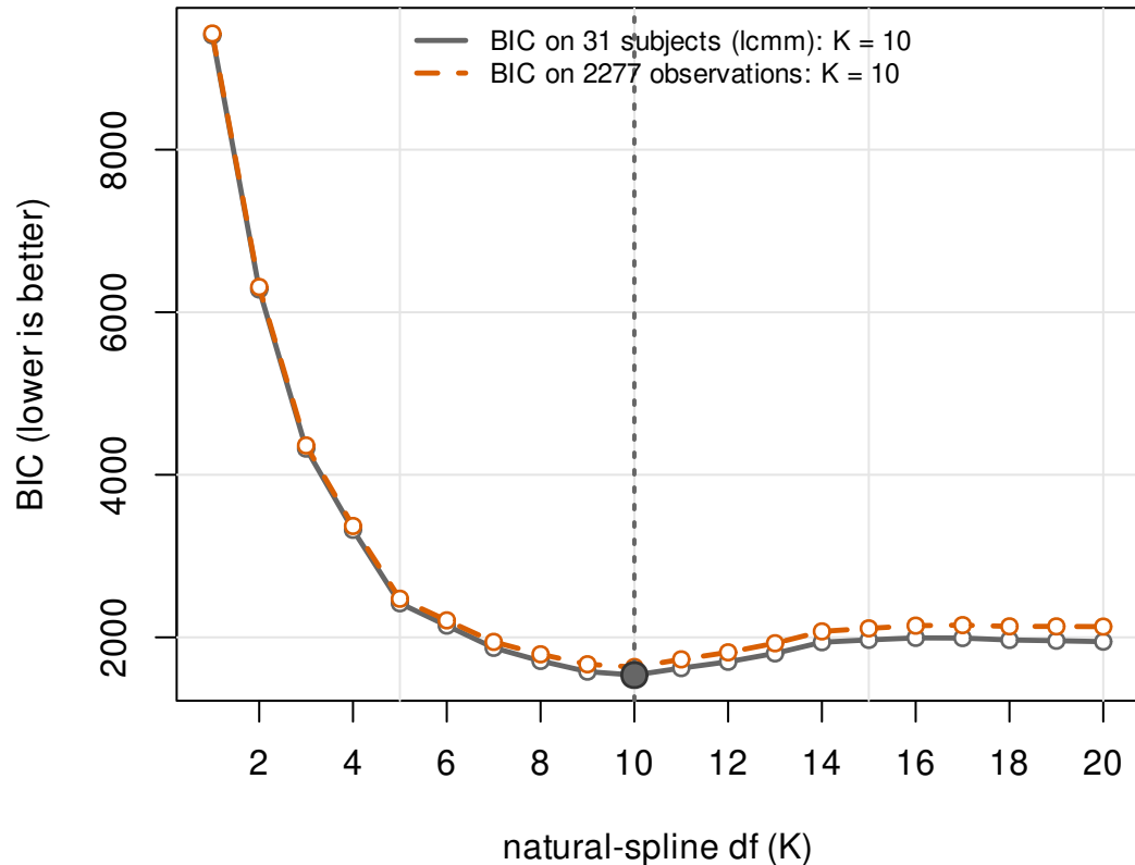
BIC turns — and where does not depend on what n means
