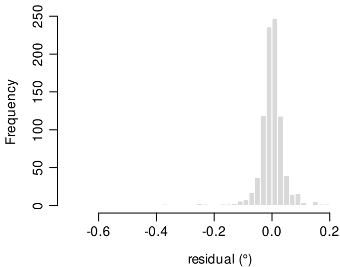
residual distribution
