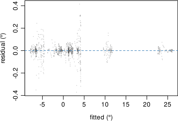
residual distribution
