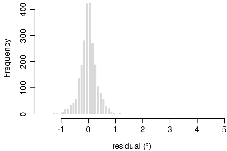
residual distribution
