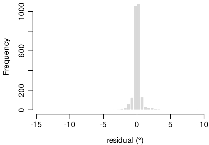
residual distribution
