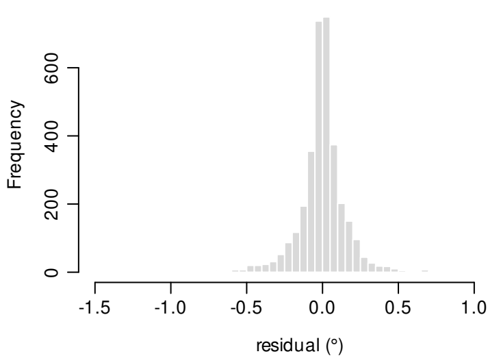
residual distribution
