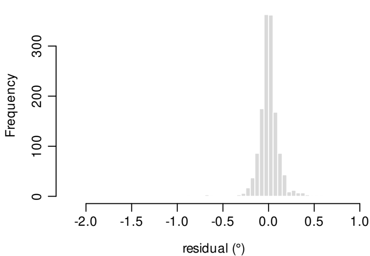
residual distribution
