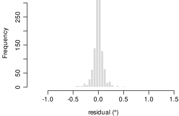
residual distribution
