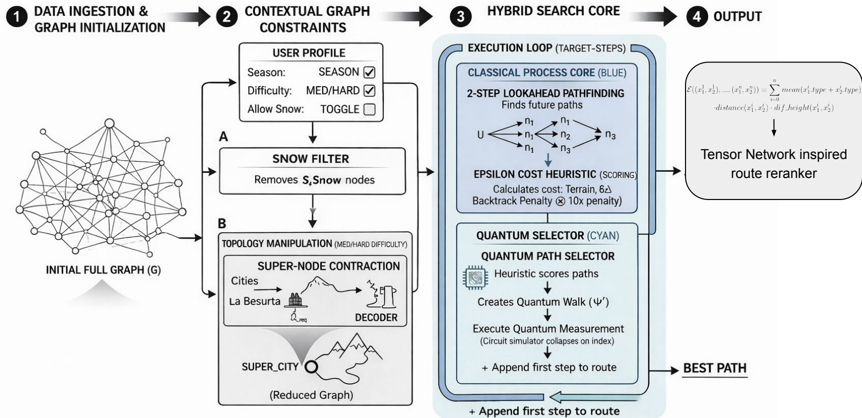
FIGURE 1: Simplified Diagram of the Hybrid Quantum-Classical Hike Optimization Pipeline.
