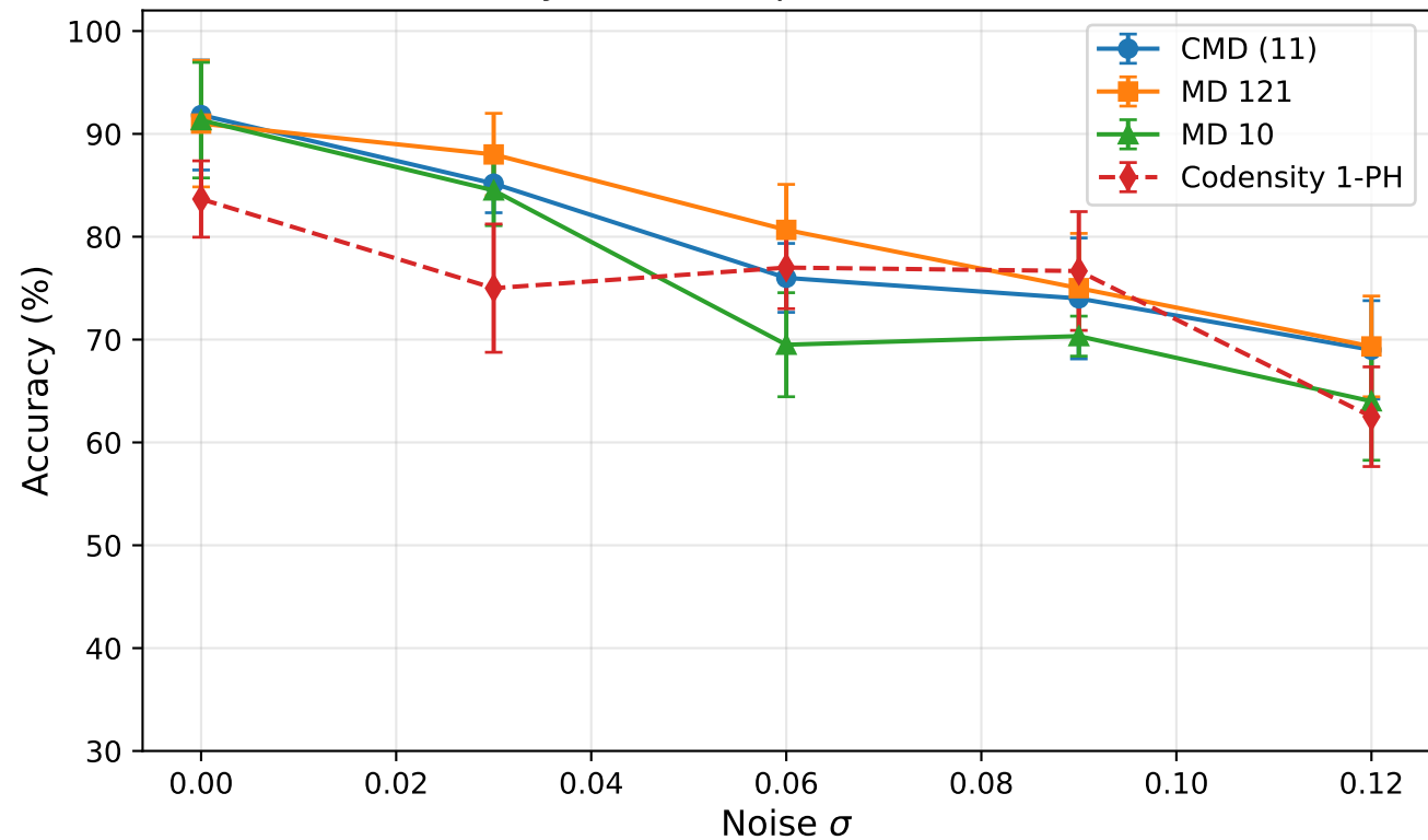
Synthetic shapes — n = 500
