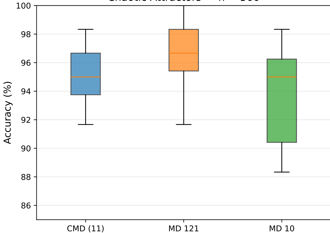
Chaotic Attractors — n = 500
