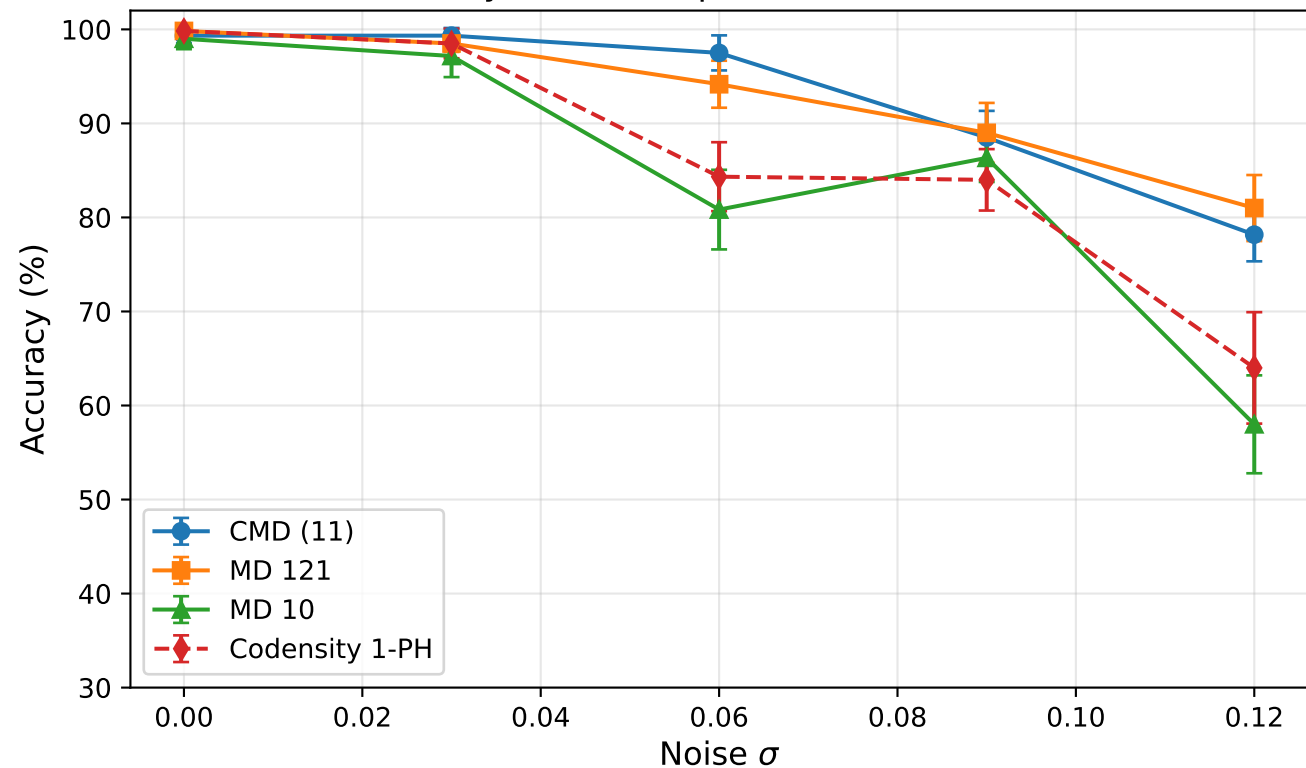
Synthetic shapes — n = 5000
