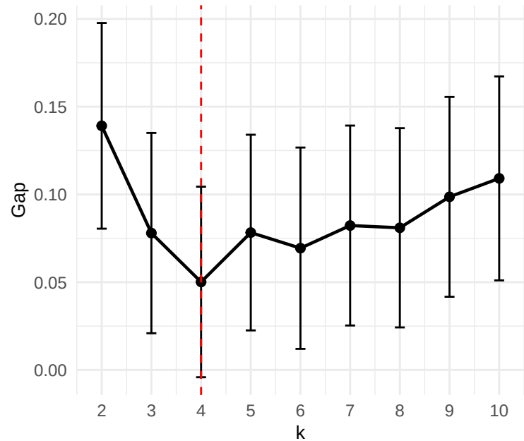
Gap Statistic
