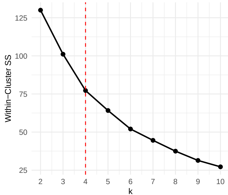
Elbow Plot (WSS)
