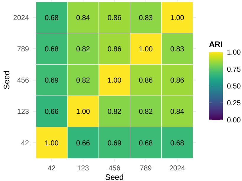
5x5 (mean ARI=0.773)
