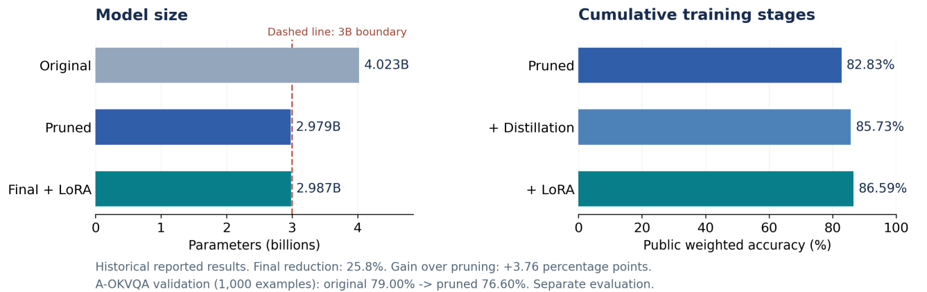
Figure 2. Parameter counts and public leaderboard scores are plotted separately; the annotation also records the local A-OKVQA baseline comparison. Both plotted axes start at zero. The original model's 79.00% validation accuracy is not a public leaderboard score.
