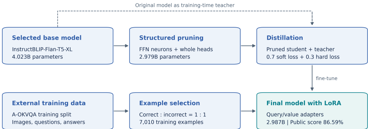
Figure 1. Structured pruning removes FFN intermediate neurons and whole decoder attention heads. The original model supplies the starting weights and the training-time teacher. Final inference uses the compressed student with LoRA adapters.
