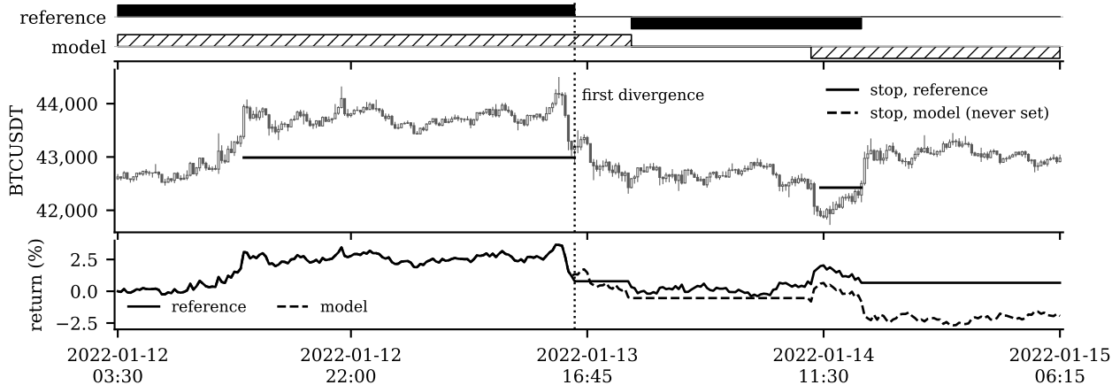
(a) GPT-5.4-mini, S0798: breakeven stop never armed
