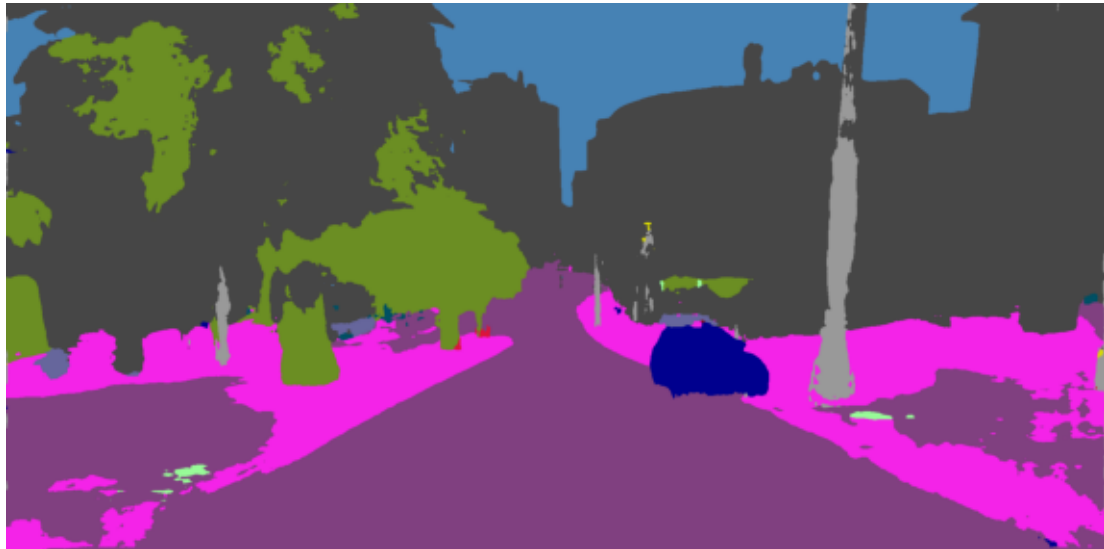
Prediction: DeepLabV3+-R101
