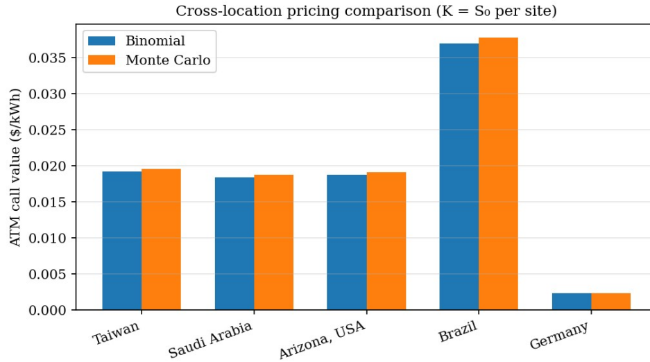
Figure 4.2. Cross-location ATM comparison.
