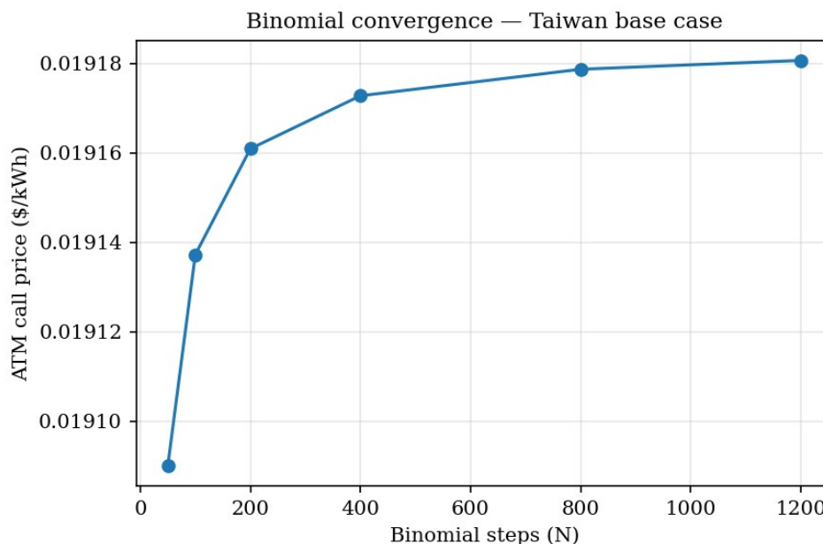
Figure 4.3. Binomial convergence (Taiwan).
