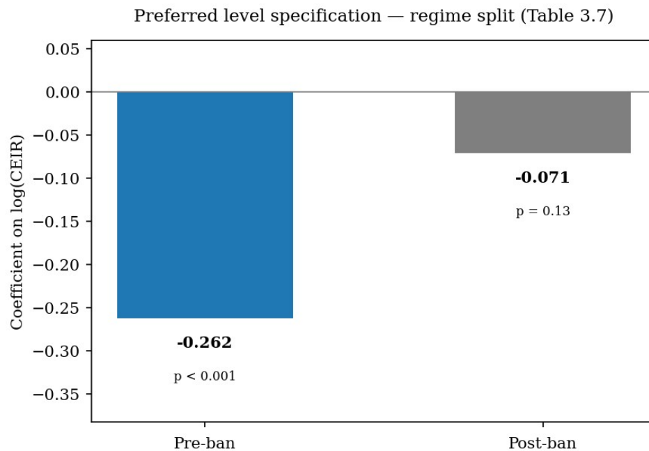
Figure 3.1. Regime split (Table 3.7). Pre-ban \beta \approx -0.26 (HAC p < 0.001 ); post-ban \beta \approx -0.07 (HAC p \approx 0.13 ). Chow break p \approx 1.1 \times 10^{-16} ; N_{\text{pre}} = 872 , N_{\text{post}} = 1,408 .
