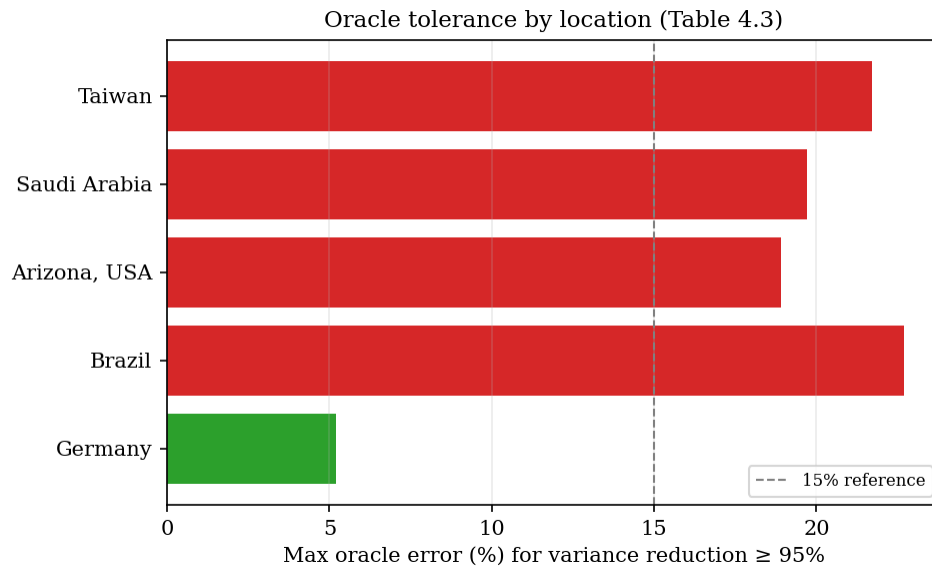
Figure 4.5. Oracle tolerance by location.
