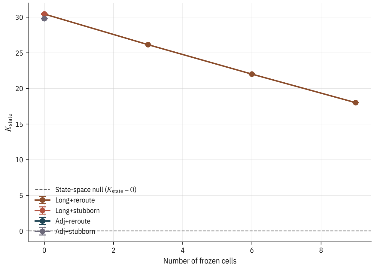
Matched state-space K under immovable frozen indices
