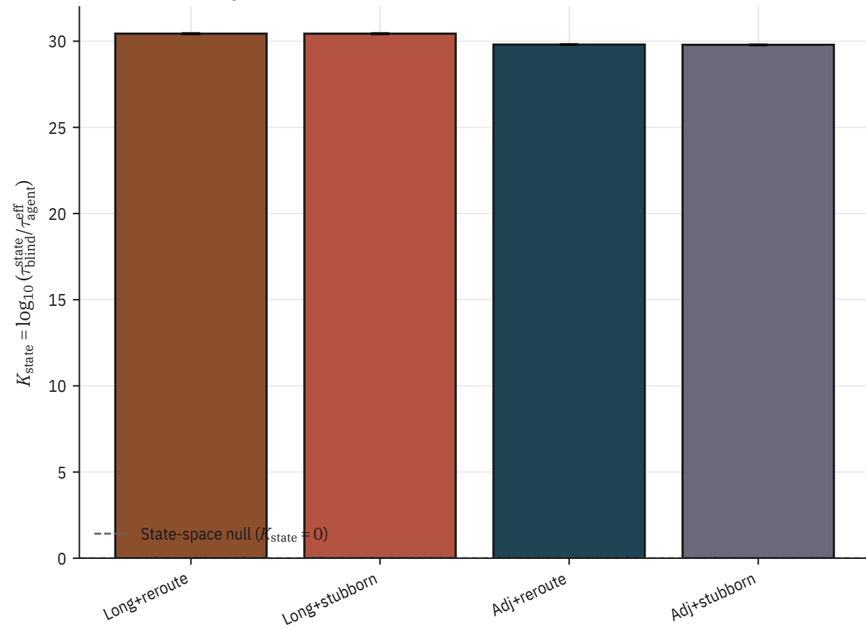
Matched state-space K at frozen=0
