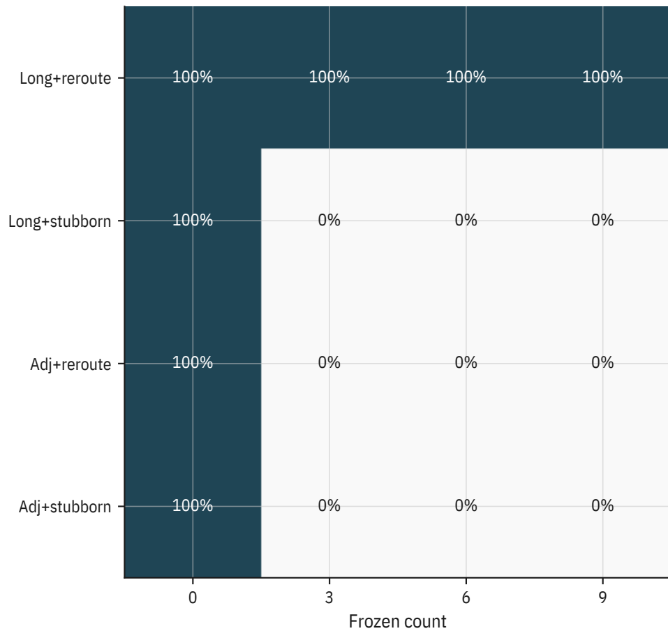
Immovable semantics
