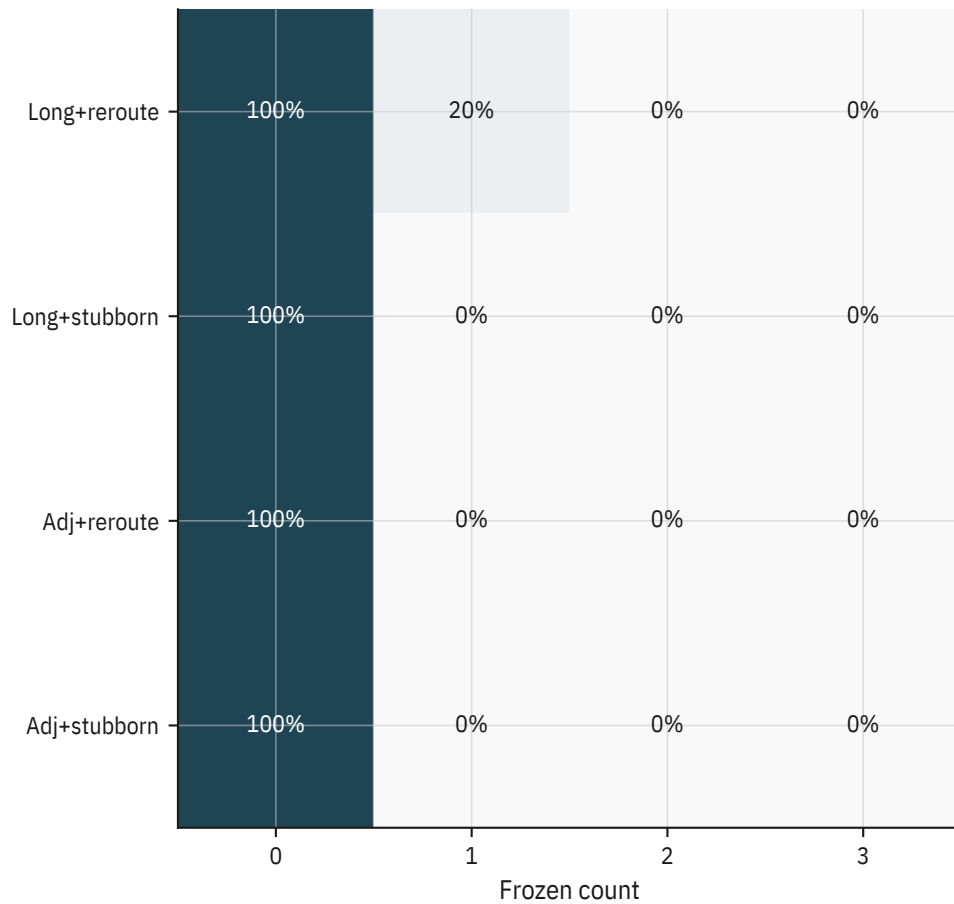
Movable semantics
