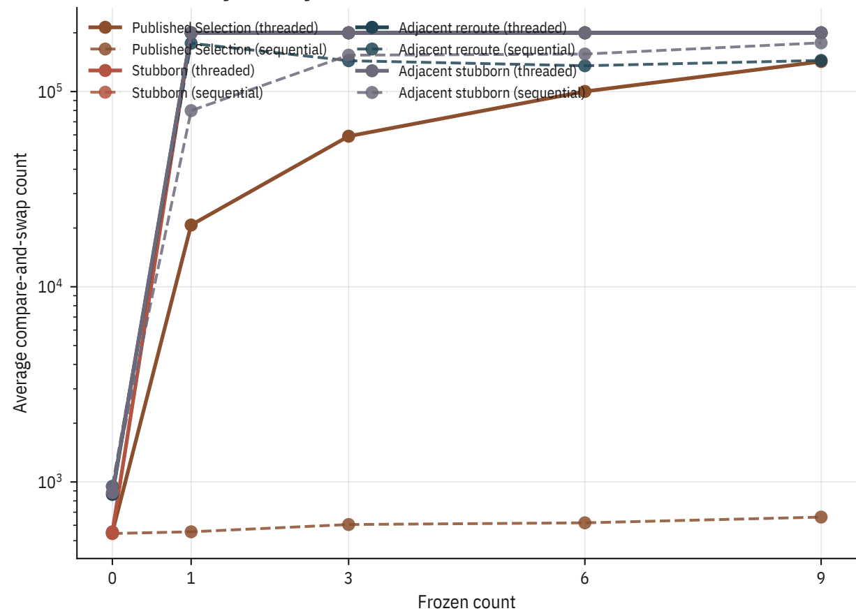
Selection-family work by substrate
