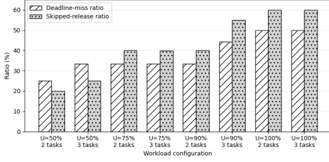
Fig. 3. Super Loop deadline-miss and skipped-release ratios for a specific task under different CPU utilization ( U ) levels and task-set sizes.
