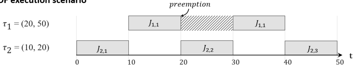
Fig. 3. EDF execution scenario for the task set in Table II. Hatching indicates a preempted job awaiting resumption.
