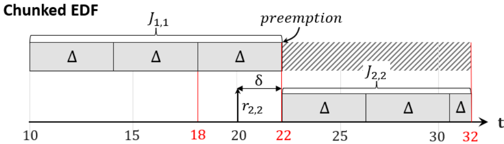
Fig. 4. Chunk-bounded preemption in the EDF implementation.
