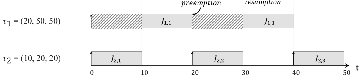
Fig. 3. EDF schedule for Table III. Arrows mark releases and hatching indicates waiting.
