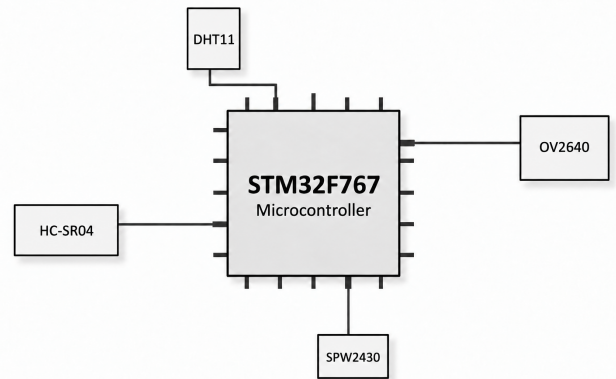
Fig. 1. Sensor platform based on STM32F767.
