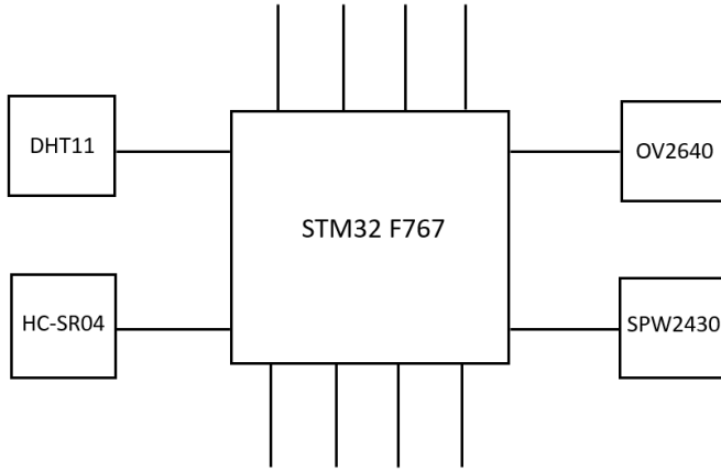
Fig. 1. STM32 hardware platform and connected sensors.
