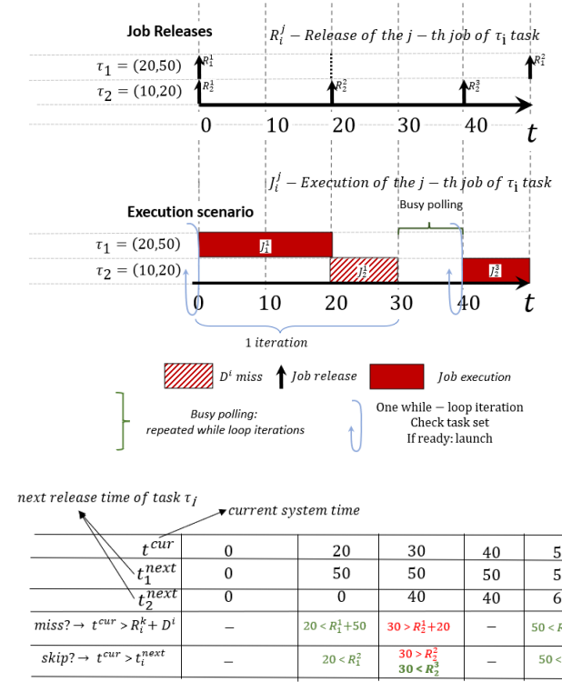
Fig. 2. Super Loop execution scenario and corresponding scheduling state.
