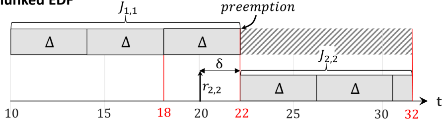
Fig. 4. Chunk-bounded preemption in the EDF implementation.
