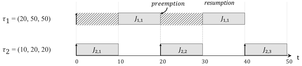
Fig. 3. EDF schedule for Table II. Arrows mark releases and hatching indicates waiting.
