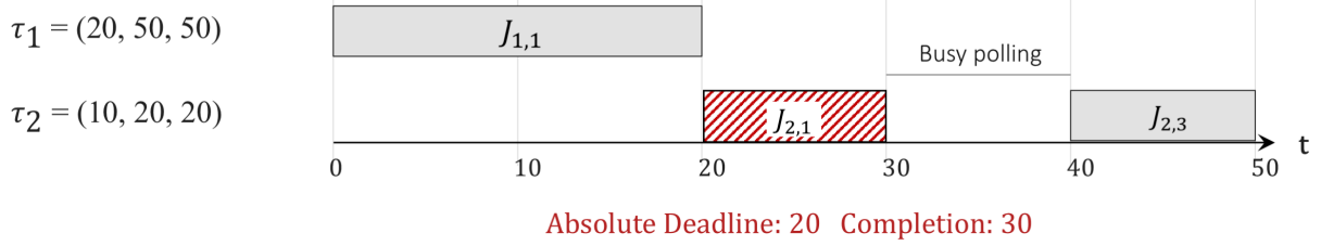
Fig. 2. SuperLoop execution scenario for the task set in Table II. Hatching indicates execution after the deadline.
