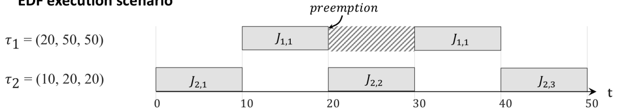
Fig. 3. EDF execution scenario for the task set in Table II. Hatching indicates a preempted job awaiting resumption.
