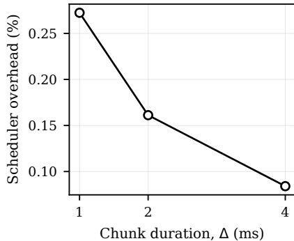
(a) Scheduler overhead
