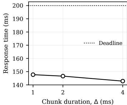
(c) \tau_3 response time
