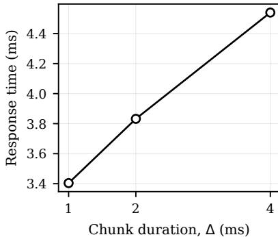
(b) \tau_1 response time
