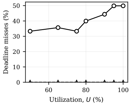
(a) Deadline-miss ratio
