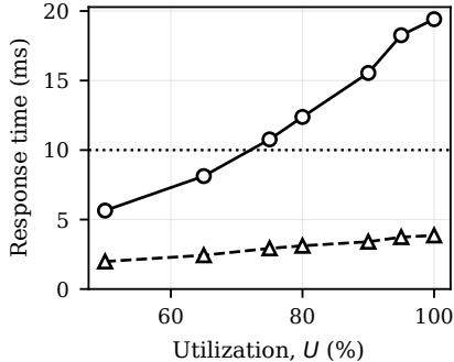
(c) Average response time
