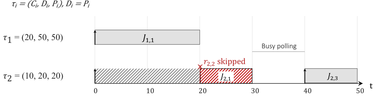
Fig. 2. SuperLoop execution scenario for the task set in Table II. Upward arrows mark releases; the crossed marker denotes a skipped release. Gray hatching indicates waiting; red hatching indicates execution after the deadline.
