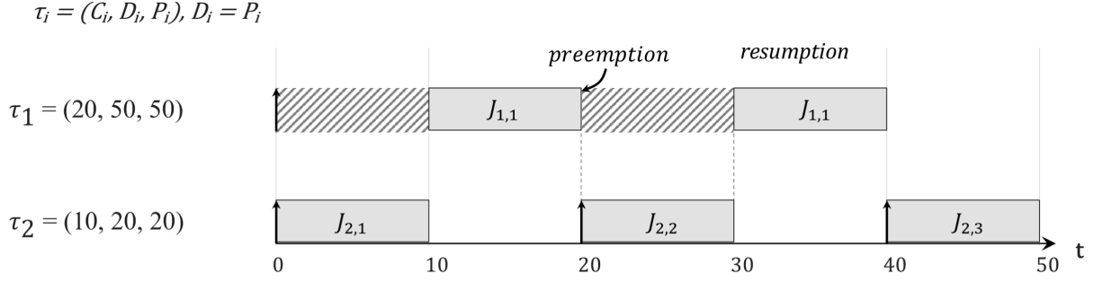
Fig. 3. EDF execution scenario for the task set in Table II. Upward arrows mark releases. Hatching indicates a released job awaiting execution, including after preemption.
