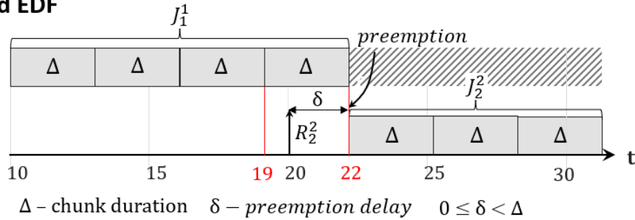
Fig. 4. Chunk-bounded preemption in the EDF implementation.
