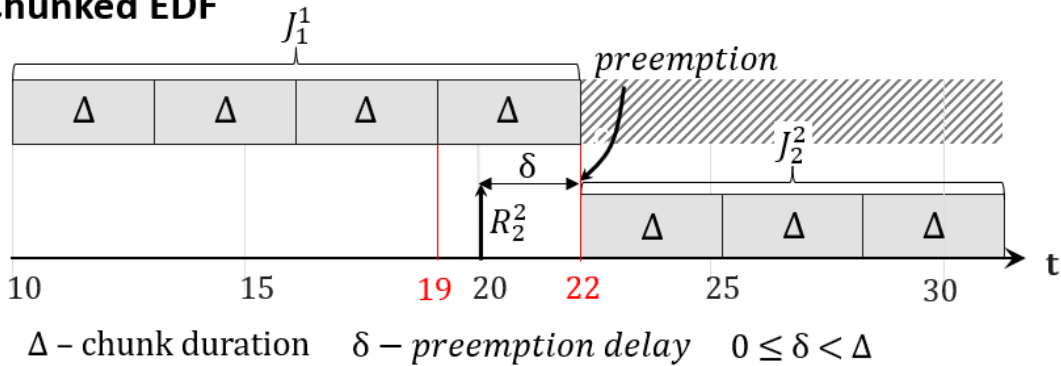
Fig. 4. Chunk-bounded preemption in the EDF implementation.
