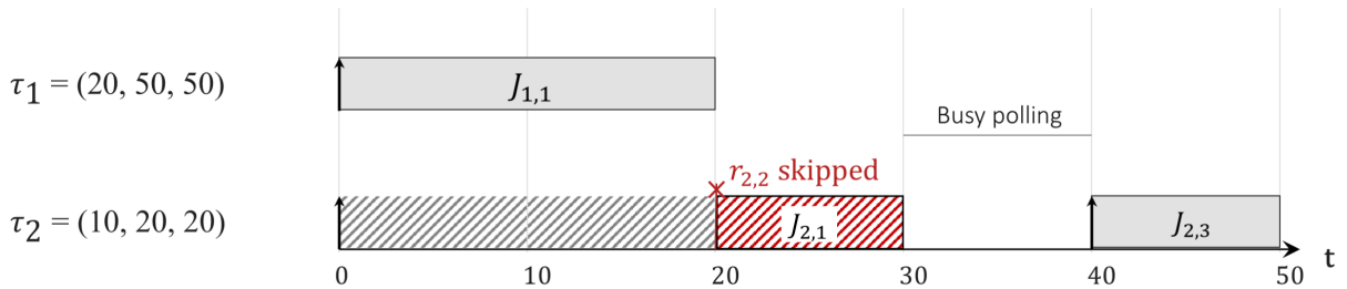
Fig. 2. SuperLoop schedule for Table III. Arrows mark releases and the cross marks a skipped release. Gray hatching indicates waiting and red hatching indicates execution after the deadline.
