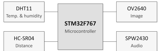
Fig. 1. Sensor platform based on STM32F767.
