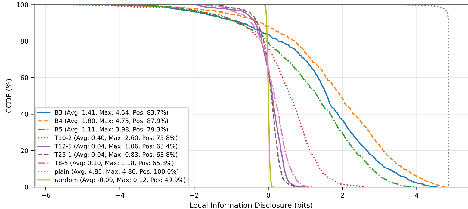
Combined Local Information Disclosure CCDF
