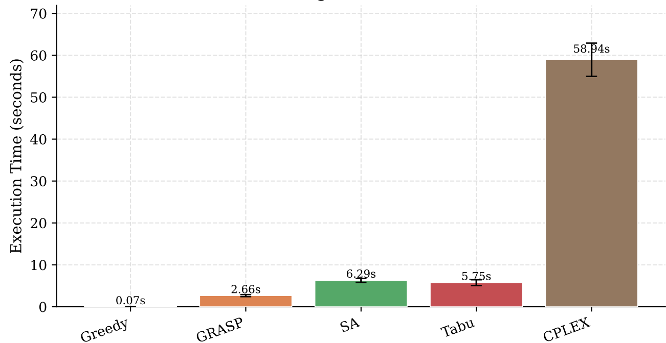
Solomon-100 -- Average Execution Time (5 instances)
