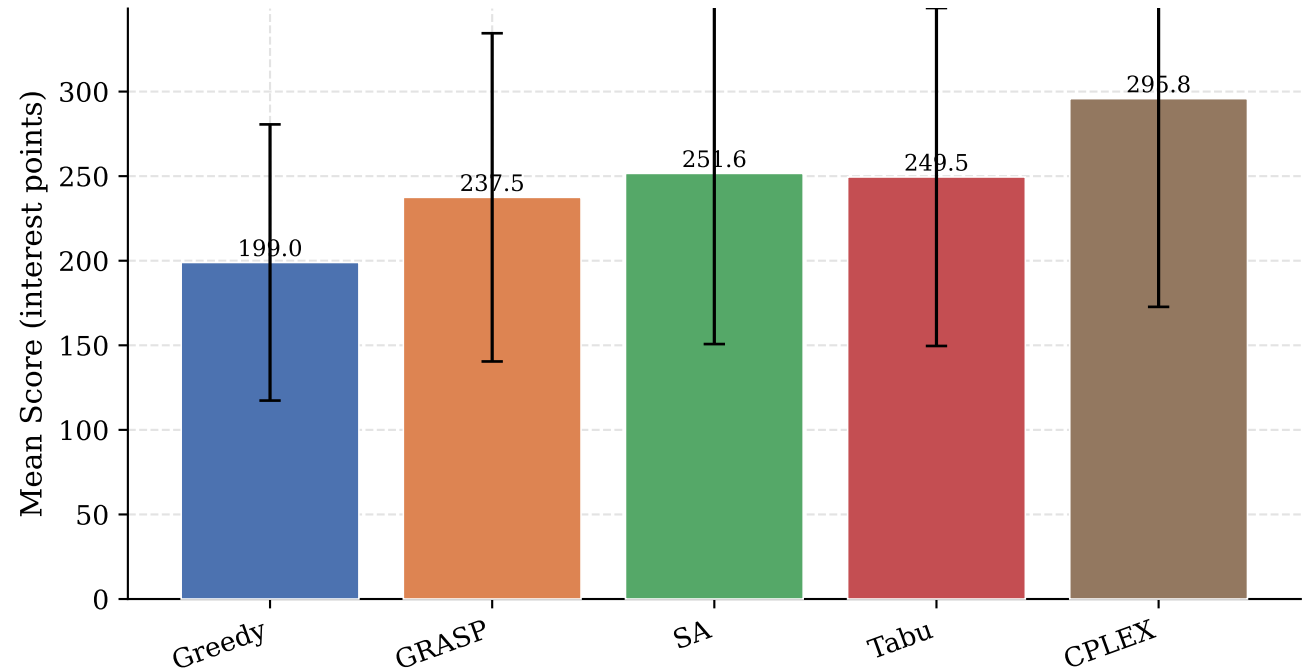
Solomon-50 -- Average Score (5 instances)
