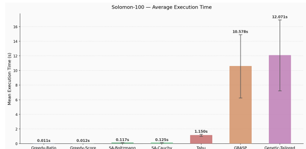
Figure 7: Mean execution time per solver on Solomon-100 [17] (error bars: \pm 1\sigma ).
