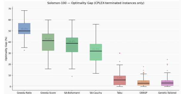
Figure 9: Optimality gap on Solomon-100 [17] (Righini & Salani [16] ground truth).
