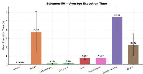
Figure 6: Mean execution time per solver on Solomon-50 [18] (error bars: \pm 1\sigma ).
