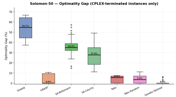
Figure 5: Optimality gap on Solomon-50 [18] (CPLEX-terminated instances only).
