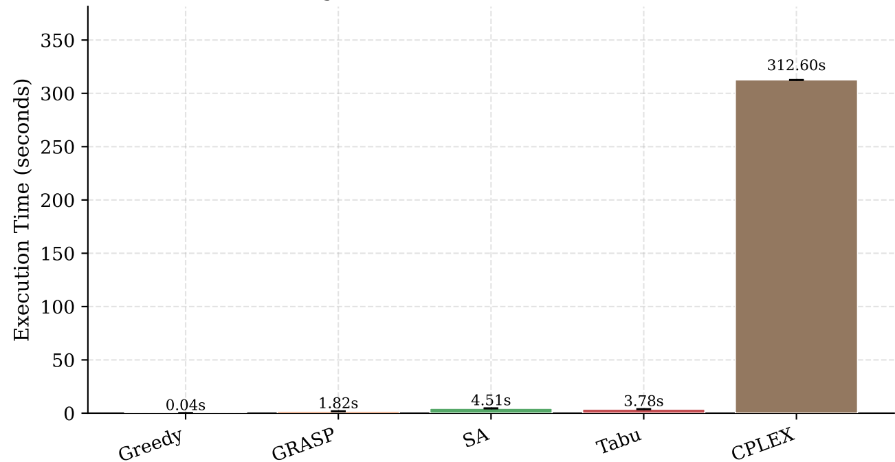
Algiers Dataset -- Execution Times
