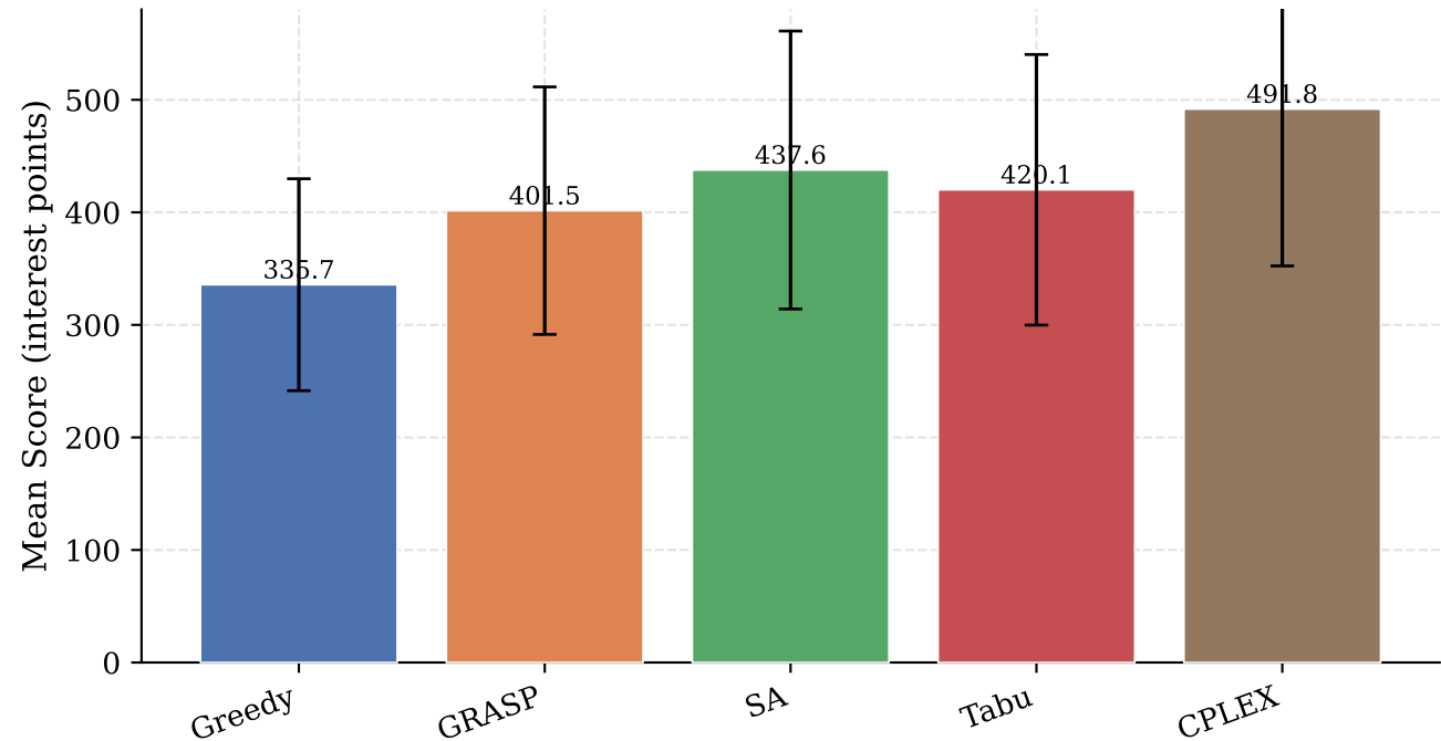
Solomon-100 -- Average Score (5 instances)
