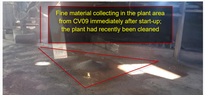
CV09-REF-002 — wet-fines/slurry consequence below the discharge/cleaner region.
