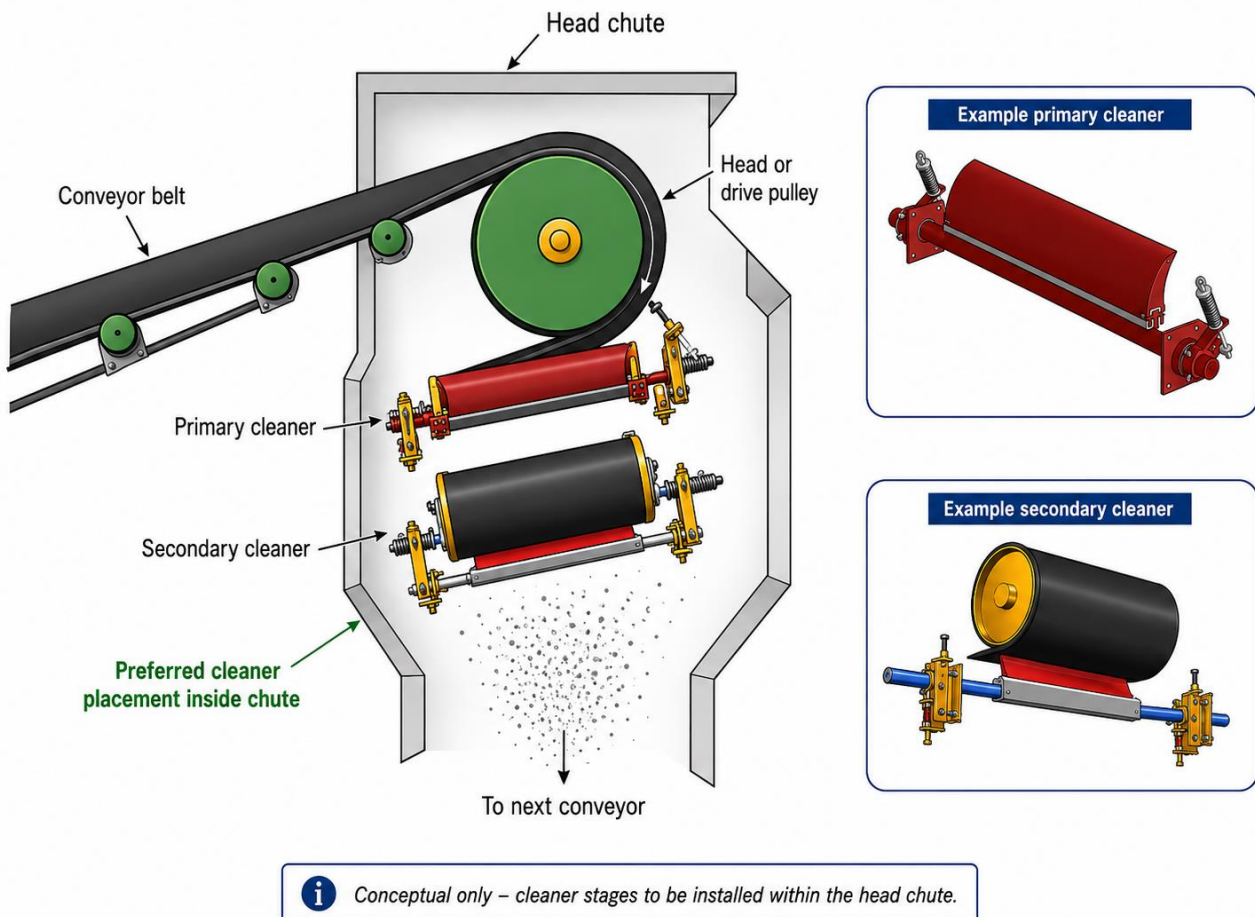
Figure 3 — CV09 Cleaners Inside Head-Chute Containment Principle (CTD-006 / DRAW-006)
