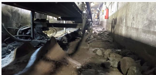
W10-REF-006 — mixed coarse product and fines distributed below the conveyor around components within the restricted tunnel area.
