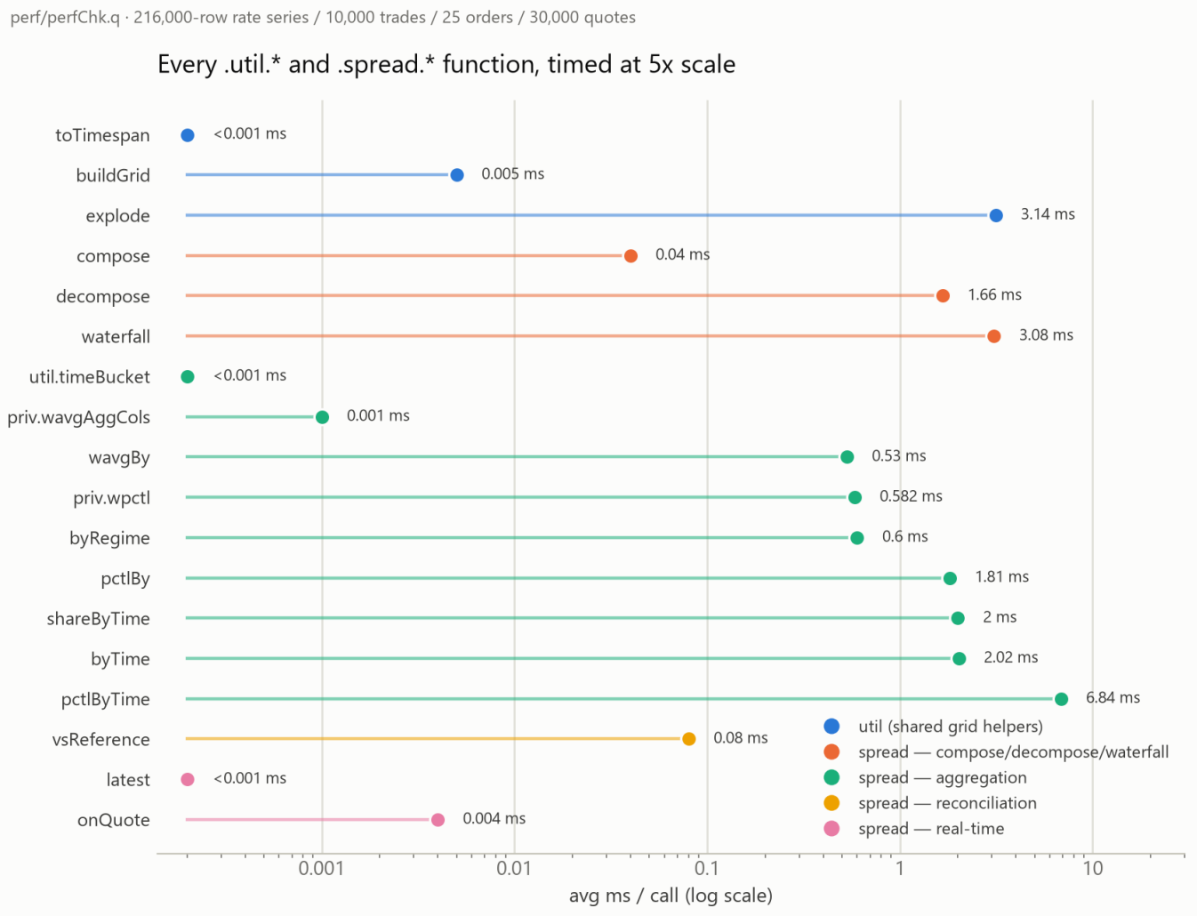
Every .util.* and .spread.* function, timed at 5x scale
