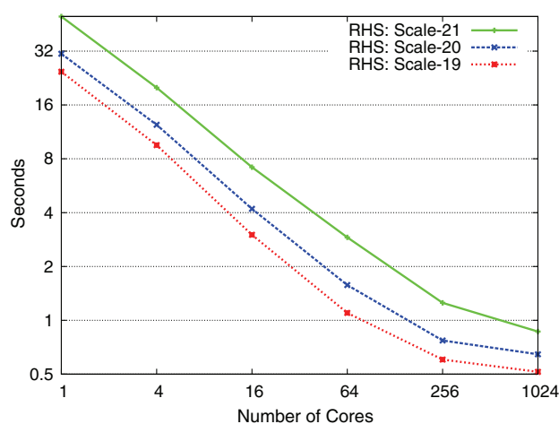
FIG. 5.3. Observed scaling of the SpAsgn operation \mathbf{A}(l, l) = \mathbf{B} where \mathbf{A} \in \mathbb{R}^{n \times n} is an R -MAT matrix of scale 22 and \mathbf{B} is another R -MAT matrix whose scale is shown in the figure legend. l is a duplicate-free sequence with entries randomly selected from the range 1 \dots n ; its length matches the dimensions of \mathbf{B} . Both axes are log scale.
