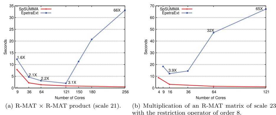
FIG. 5.13. Comparison of SpGEMM implementation of Trilinos's EpetraExt package with our Sparse SUMMA implementation using synthetically generated matrices. The data labels on the plots show the speedup of Sparse SUMMA over EpetraExt.
