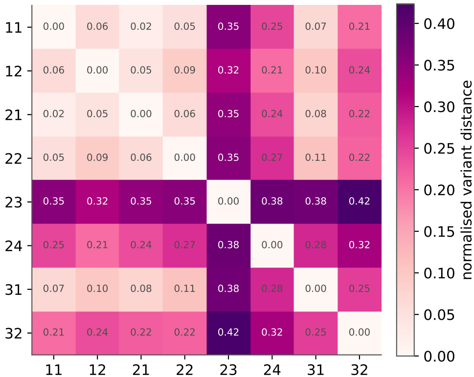
Witness distances (core block)
