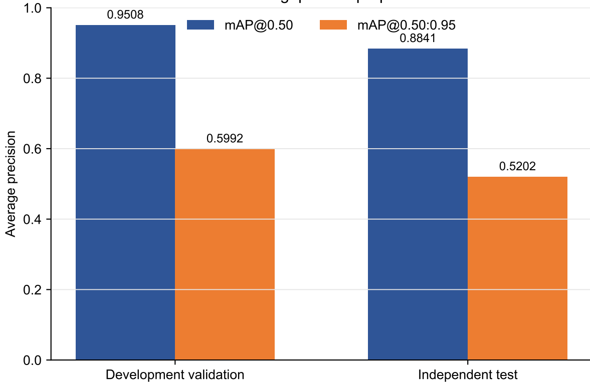
Generalization gap of the proposed fusion
